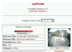
Figure 8-24. camPortal module.
