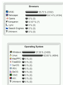
Figure 6-6. Statistics module
