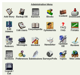
Figure 7-1. Administration panel.
